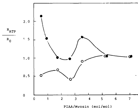
Fig.3. The effect of ATP on I_E/I_M in the presence and absence of \text{Ca}^{2+} at 0.72 \mu M myosin. The ratio of R_{\text{ATP}}/R_0 was plotted against the amount of labeled PIAA, here R_{\text{ATP}} denotes I_E/I_M in the presence of 1 mM ATP and R_0 denotes I_E/I_M in the absence of ATP. (○) In the presence of 5 mM \text{CaCl}_2 , 50 mM KCl and 50 mM Tris-HCl (pH 8.0); (●) in the presence of 5 mM EDTA, 0.5 M KCl and 50 mM Tris-HCl (pH 8.0). The fluorescences were measured immediately after the addition of ATP.
